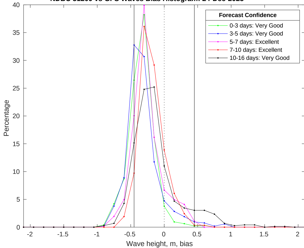
NDBC 51209 vs GFS Waves Bias Histogram: 24-Dec-2025
