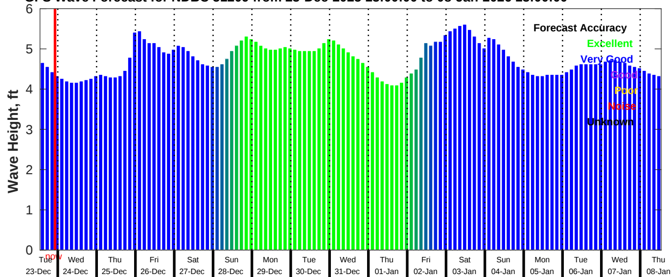
GFS Wave Forecast for NDBC 51209 from 23-Dec-2025 13:00:00 to 08-Jan-2026 13:00:00
