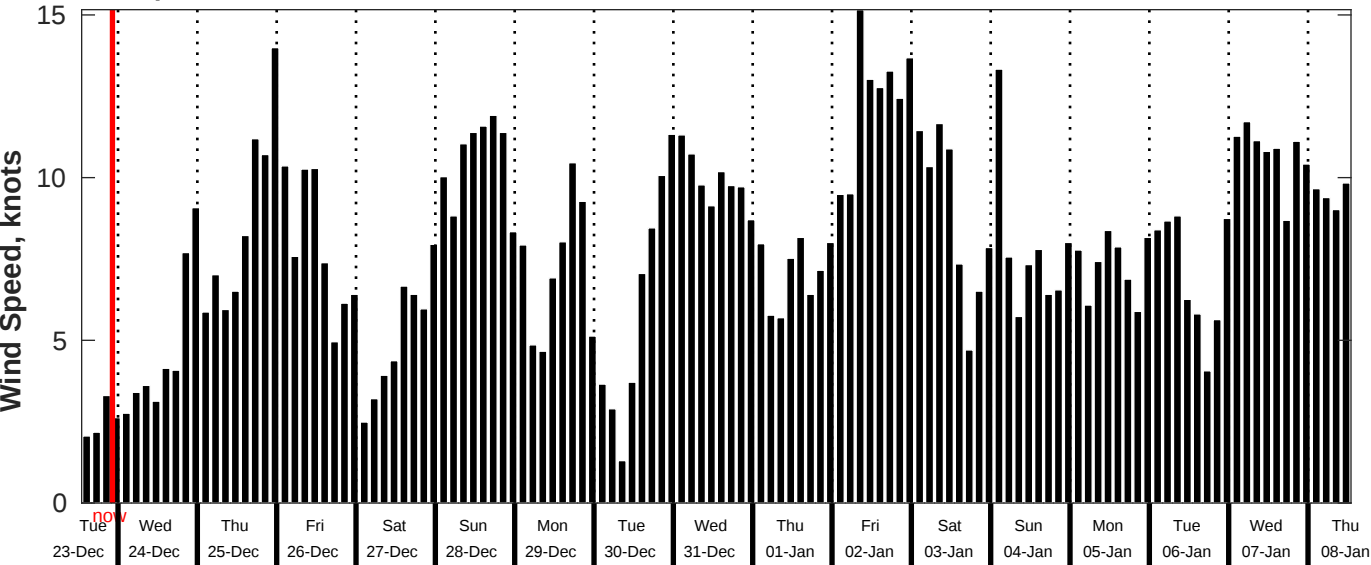
GFS Wind Speed Forecast for NDBC 51209 from 23-Dec-2025 13:00:00 to 08-Jan-2026 13:00:00
