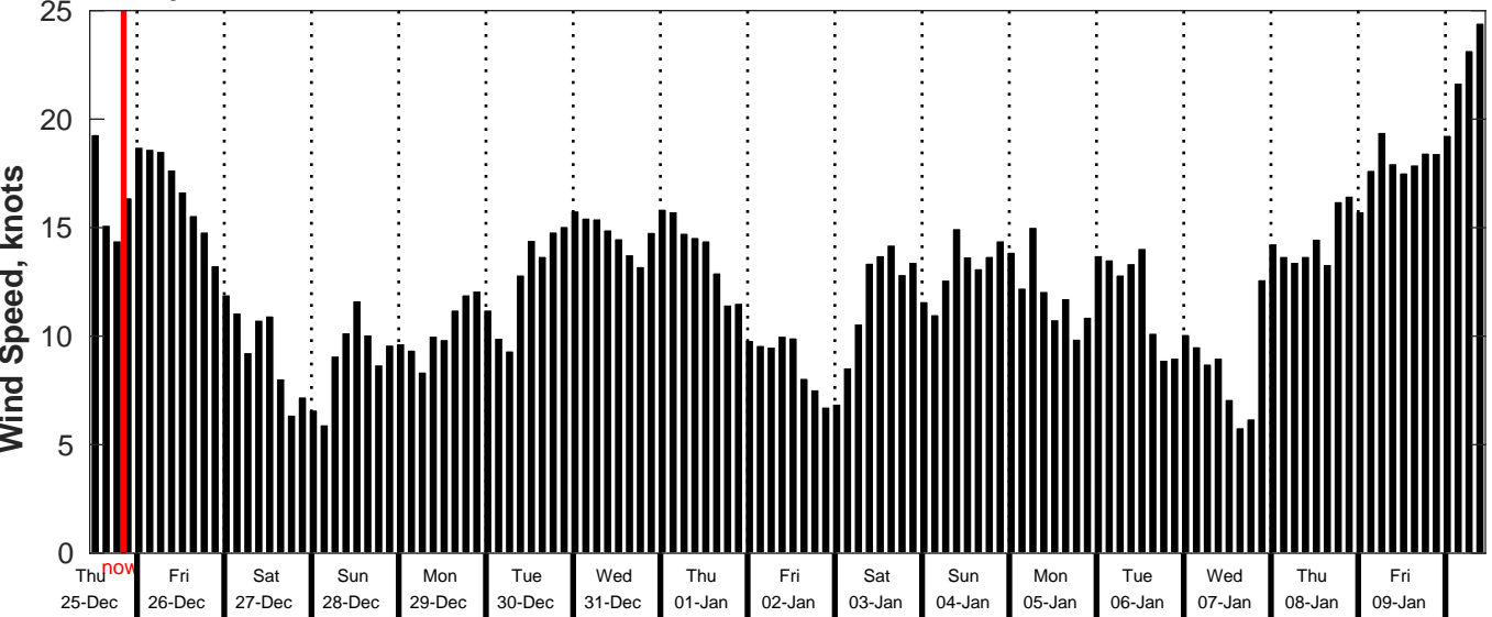
GFS Wind Speed Forecast for NDBC 52211 from 24-Dec-2025 11:00:00 to 09-Jan-2026 11:00:00
