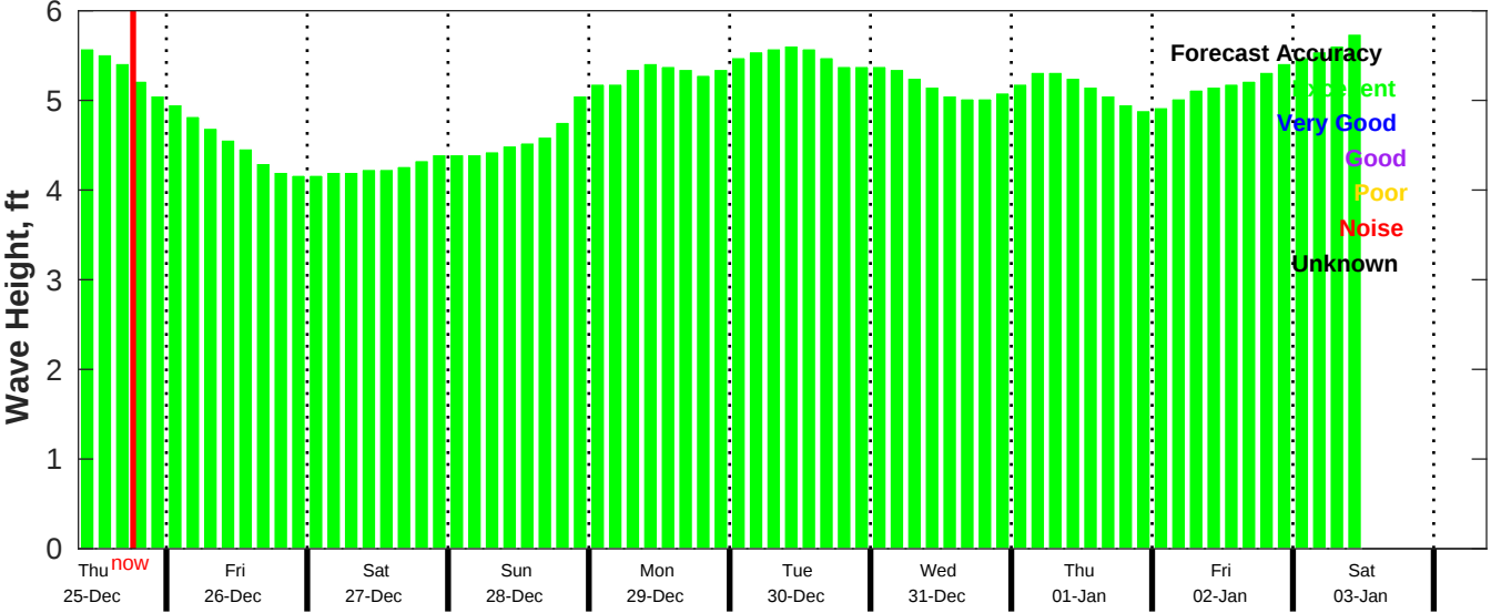
CMEMS Wave Forecast for NDBC 52212 from 24-Dec-2025 09:00:00 to 03-Jan-2026 09:00:00
