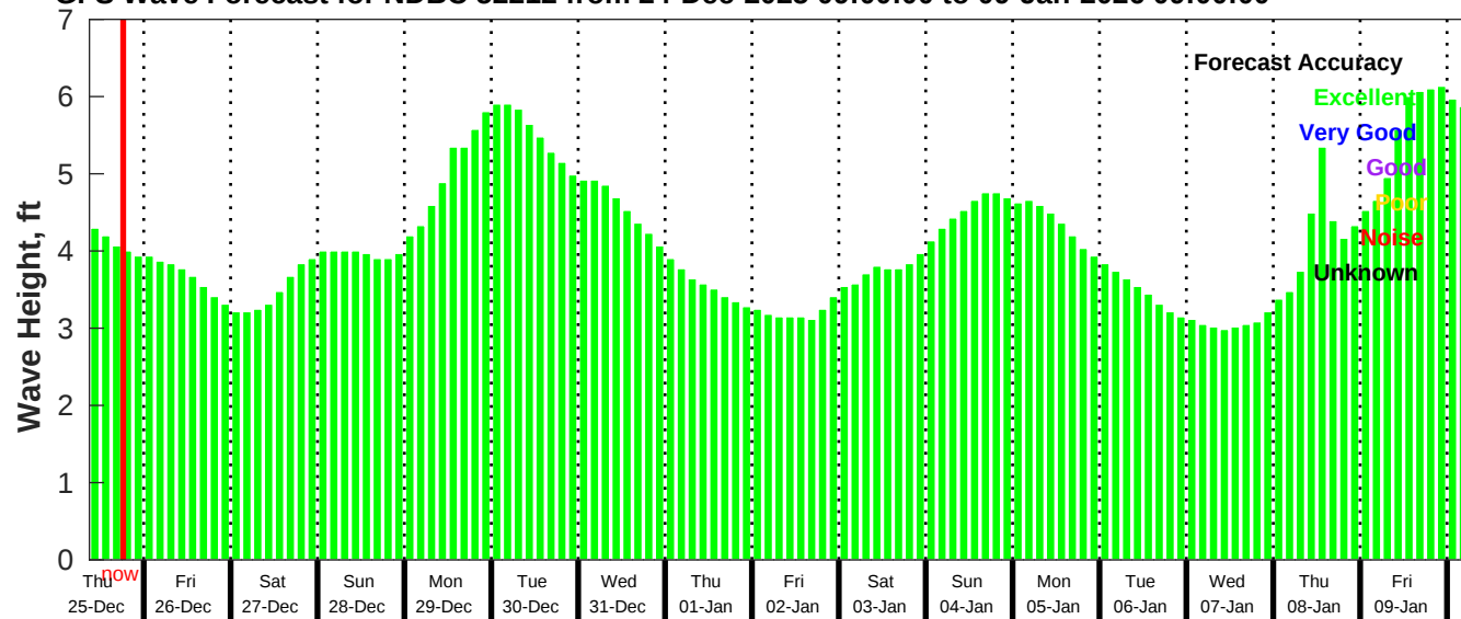
GFS Wave Forecast for NDBC 52212 from 24-Dec-2025 09:00:00 to 09-Jan-2026 09:00:00
