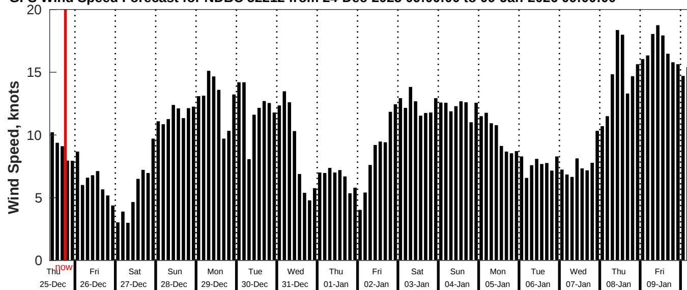
GFS Wind Speed Forecast for NDBC 52212 from 24-Dec-2025 09:00:00 to 09-Jan-2026 09:00:00
