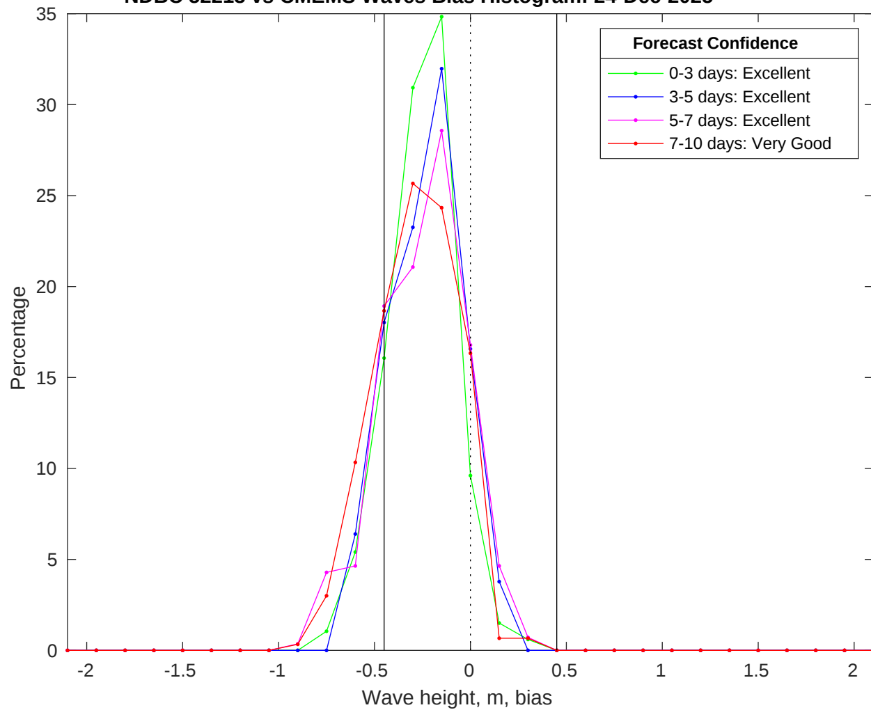
NDBC 52213 vs CMEMS Waves Bias Histogram: 24-Dec-2025
