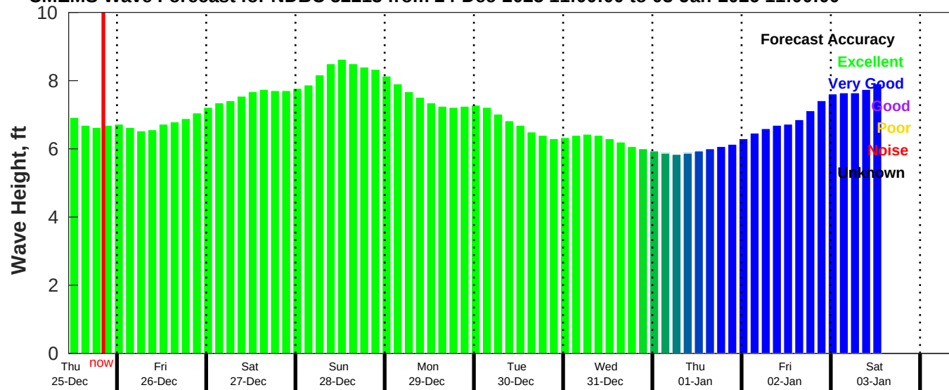
CMEMS Wave Forecast for NDBC 52213 from 24-Dec-2025 11:00:00 to 03-Jan-2026 11:00:00
