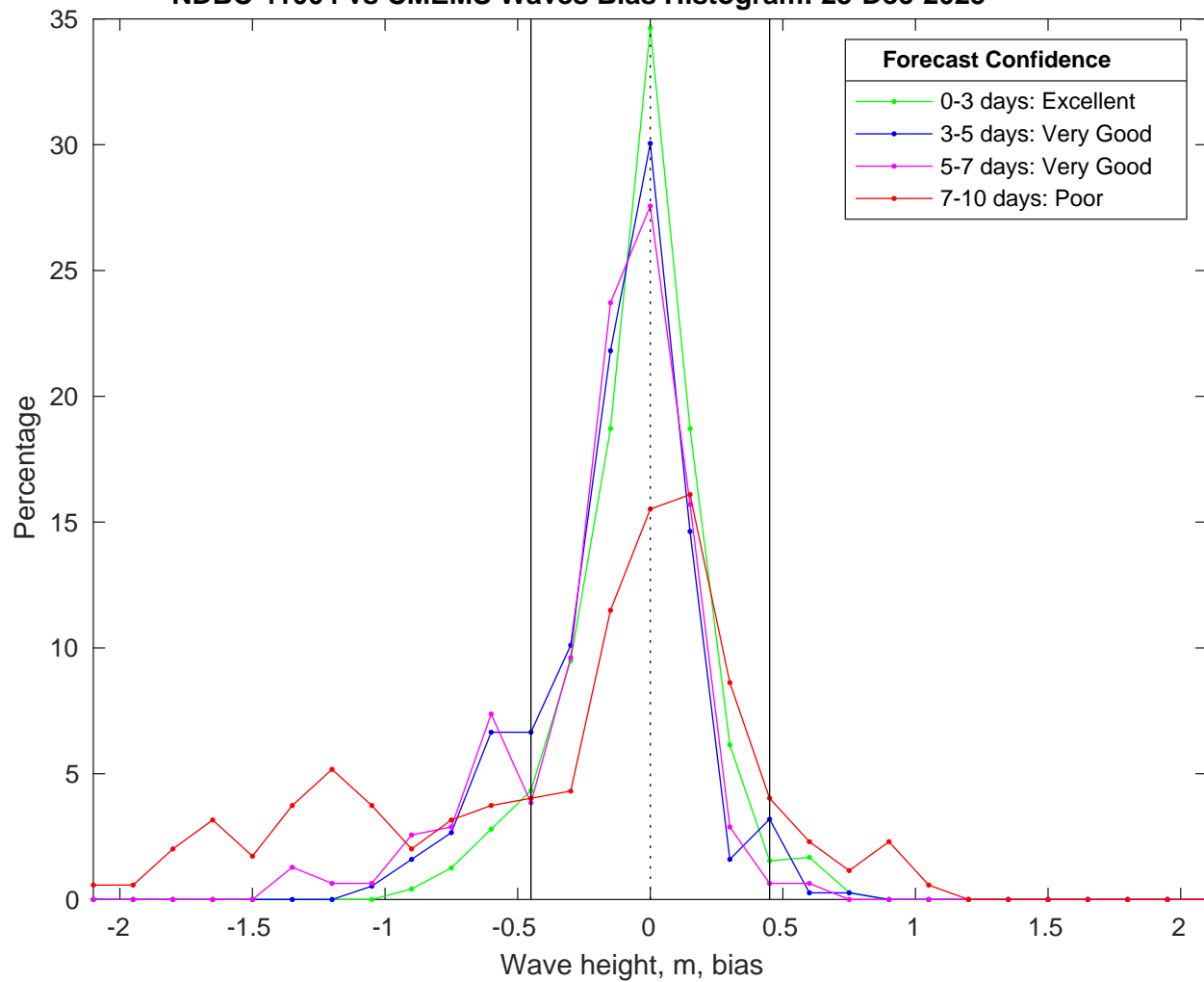
NDBC 41004 vs CMEMS Waves Bias Histogram: 25-Dec-2025
