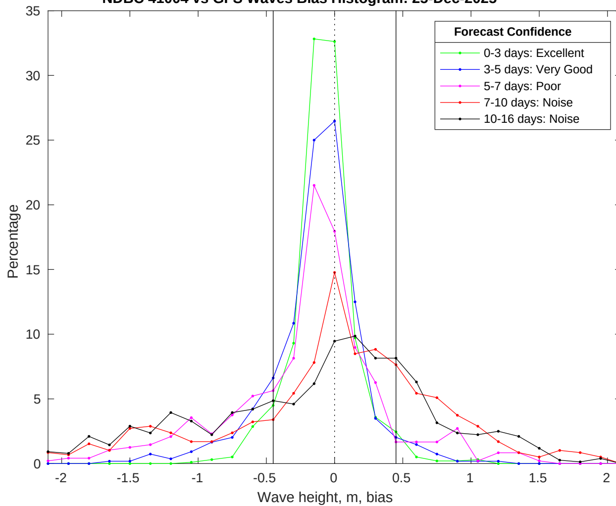
NDBC 41004 vs GFS Waves Bias Histogram: 25-Dec-2025
