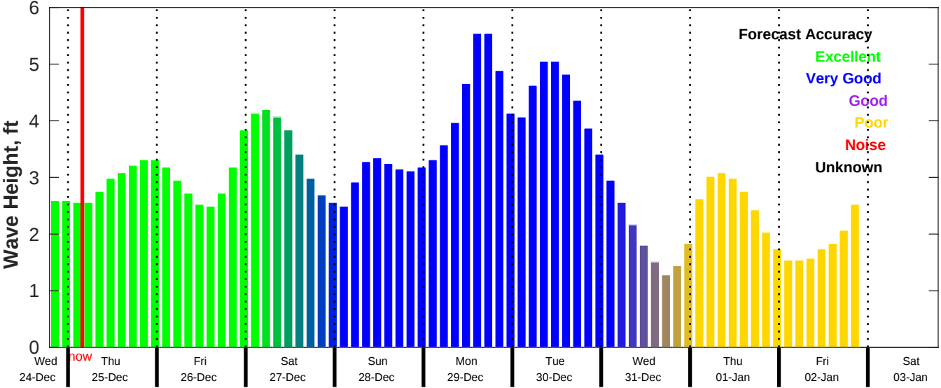
CMEMS Wave Forecast for NDBC 41004 from 24-Dec-2025 19:00:00 to 03-Jan-2026 19:00:00
