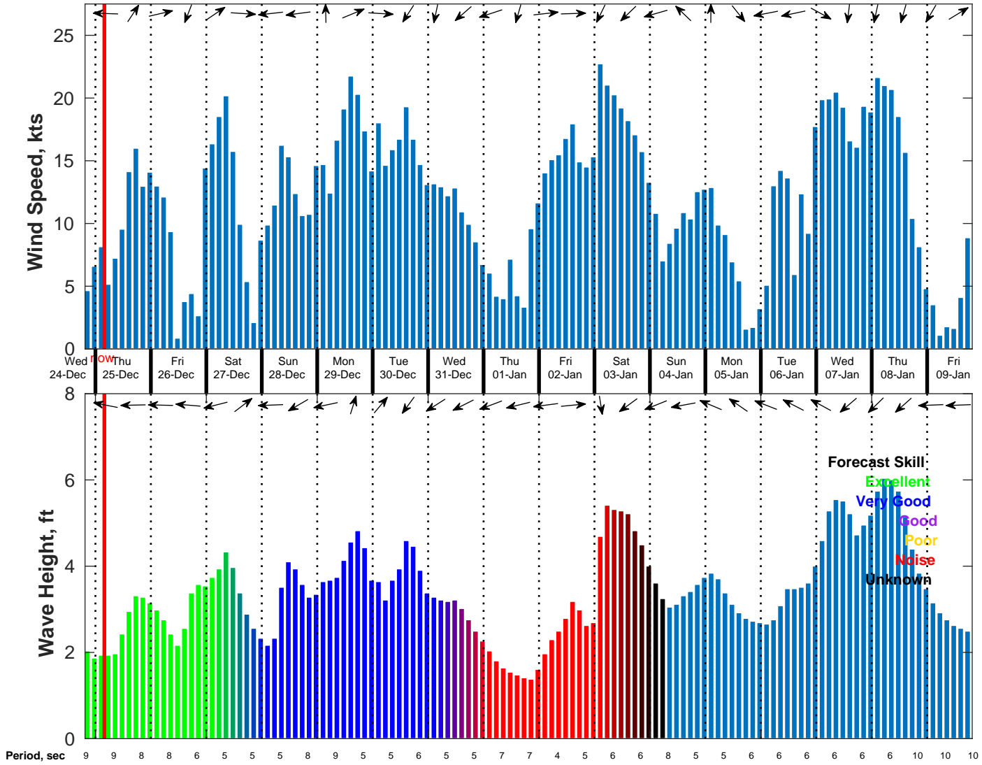
Wind & Wave Forecast for NDBC 41004 from 24-Dec-2025 19:00:00 to 09-Jan-2026 19:00:00
