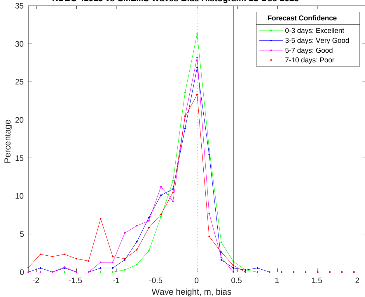
NDBC 41013 vs CMEMS Waves Bias Histogram: 25-Dec-2025
