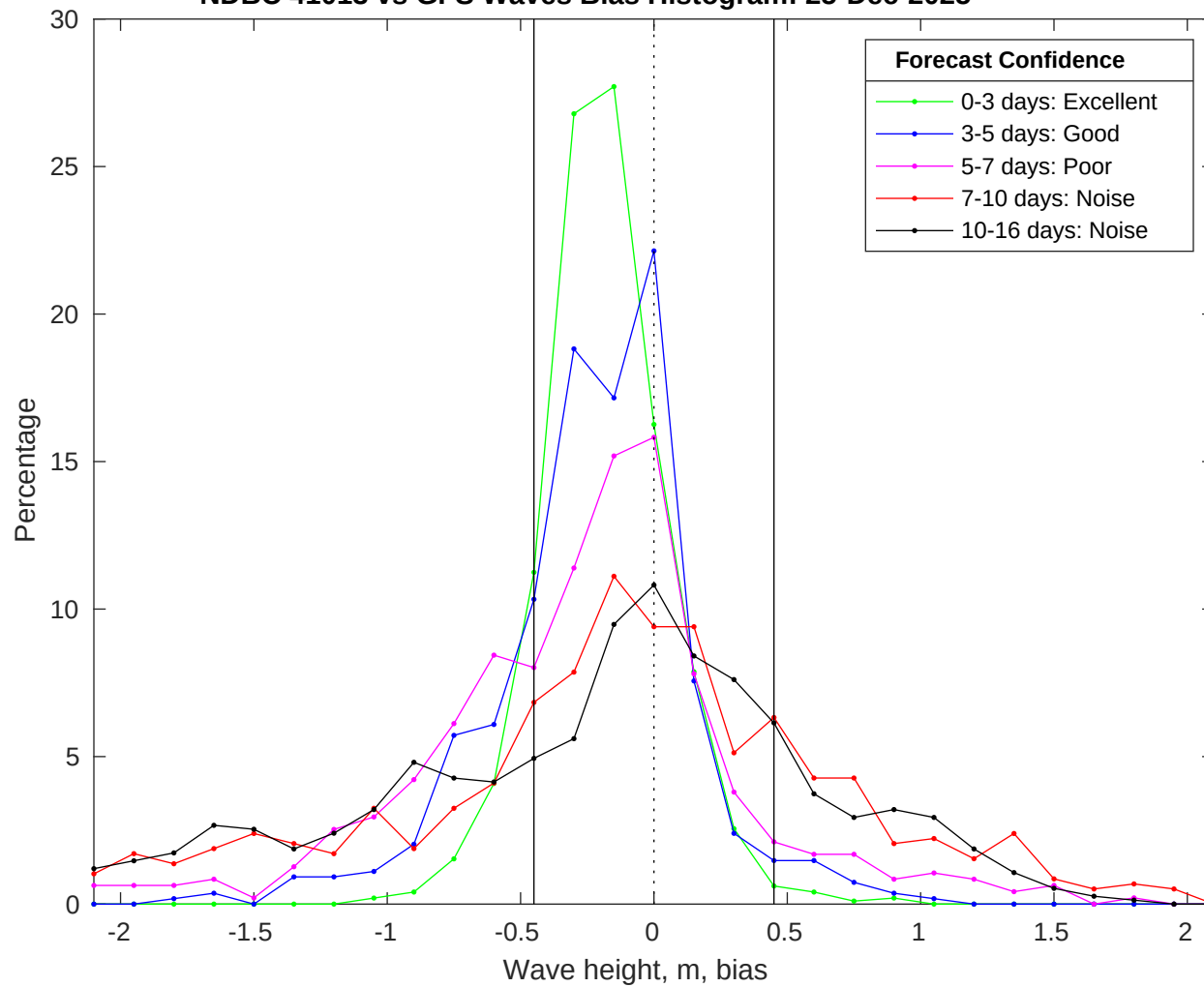
NDBC 41013 vs GFS Waves Bias Histogram: 25-Dec-2025
