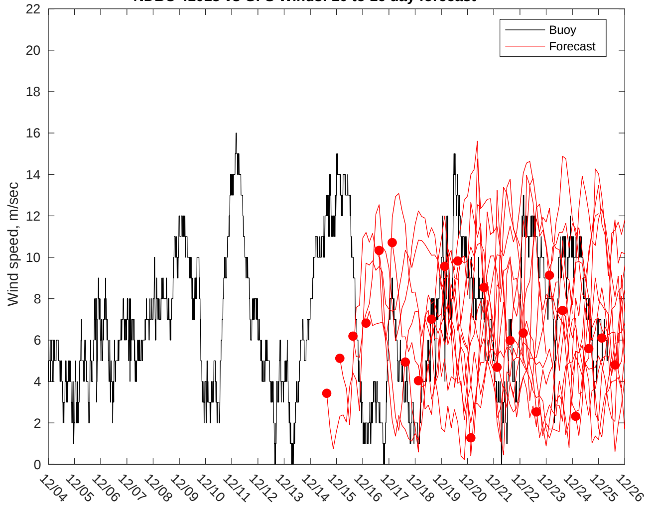
NDBC 41013 vs GFS Winds: 10 to 16 day forecast
