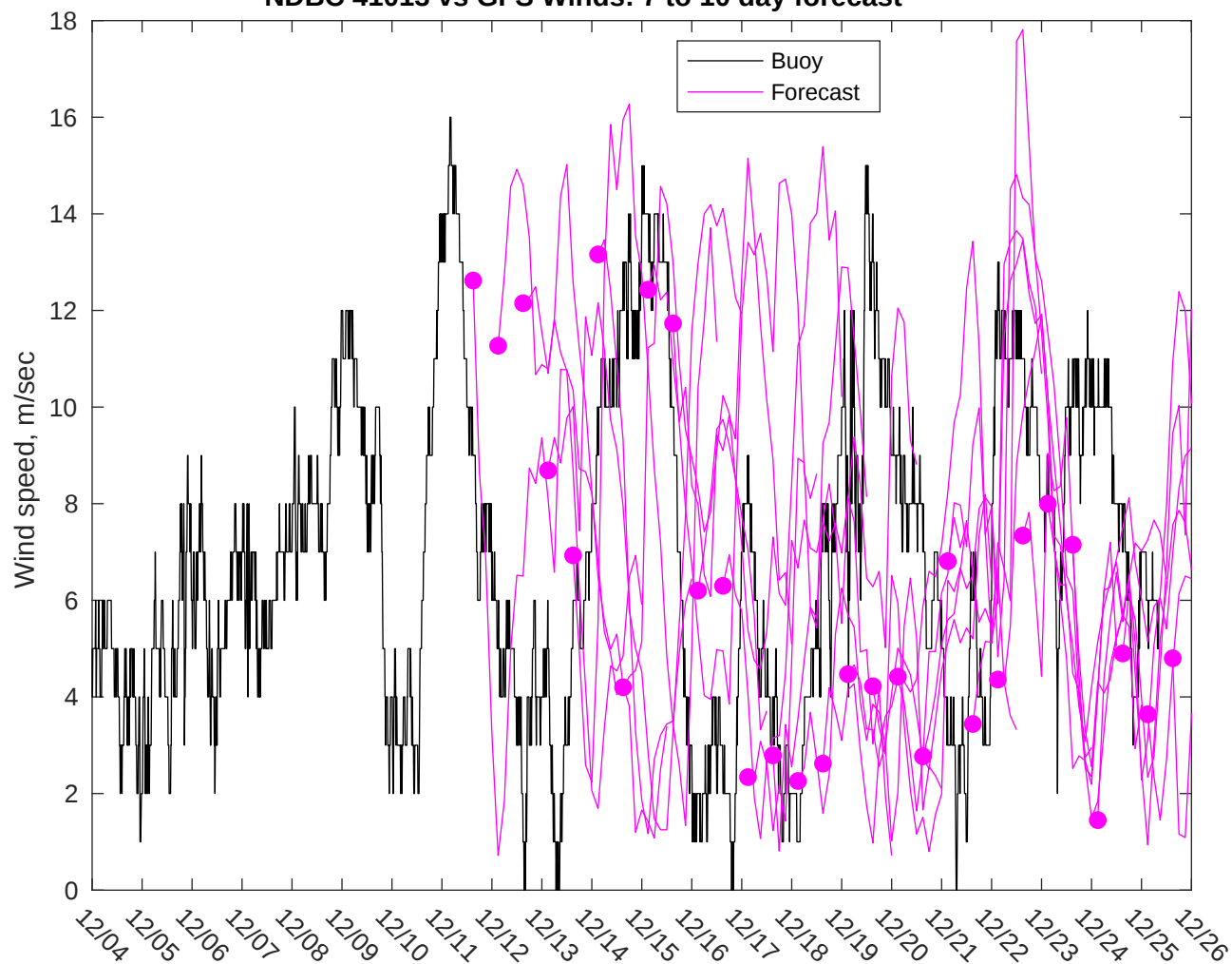
NDBC 41013 vs GFS Winds: 7 to 10 day forecast
