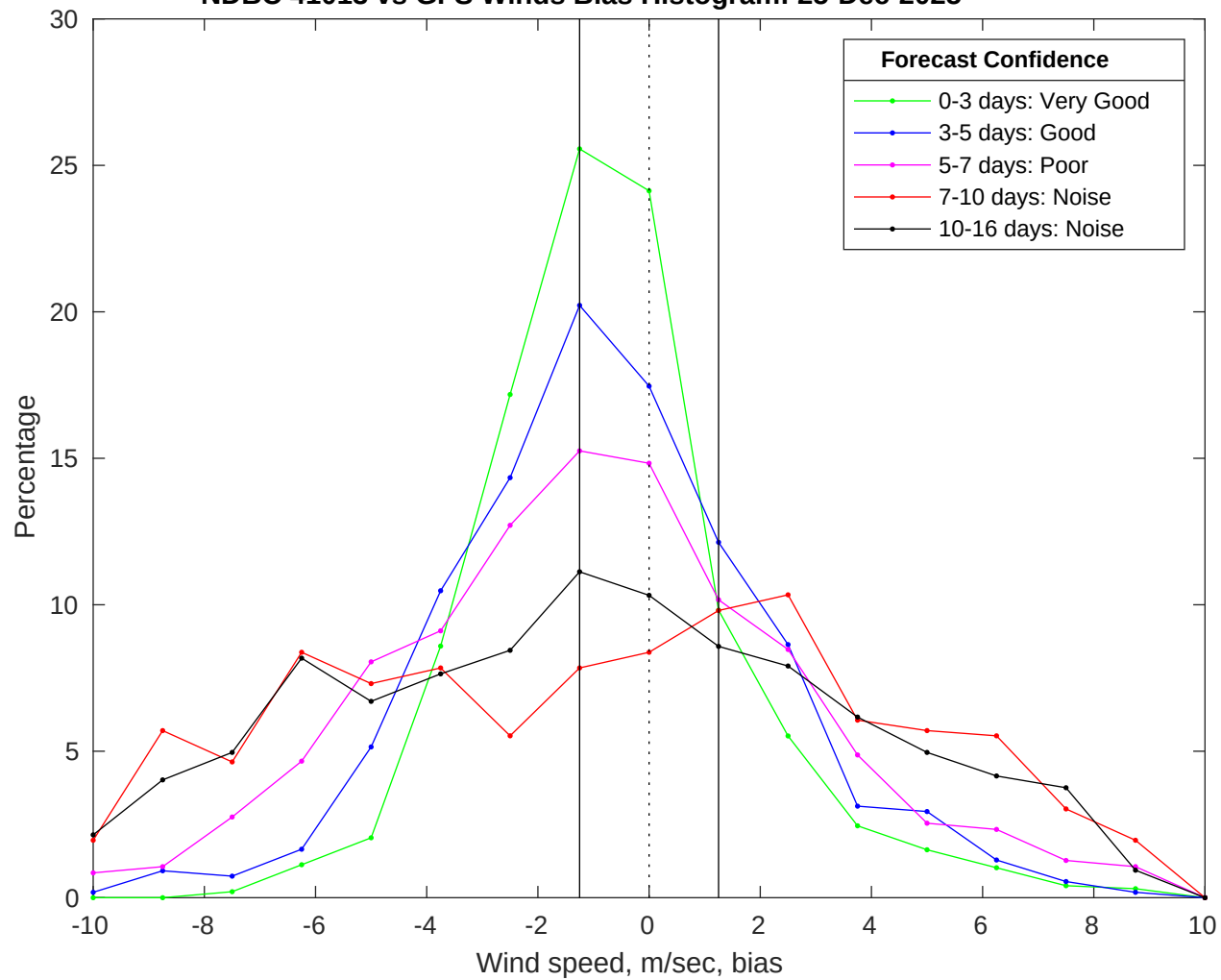
NDBC 41013 vs GFS Winds Bias Histogram: 25-Dec-2025
