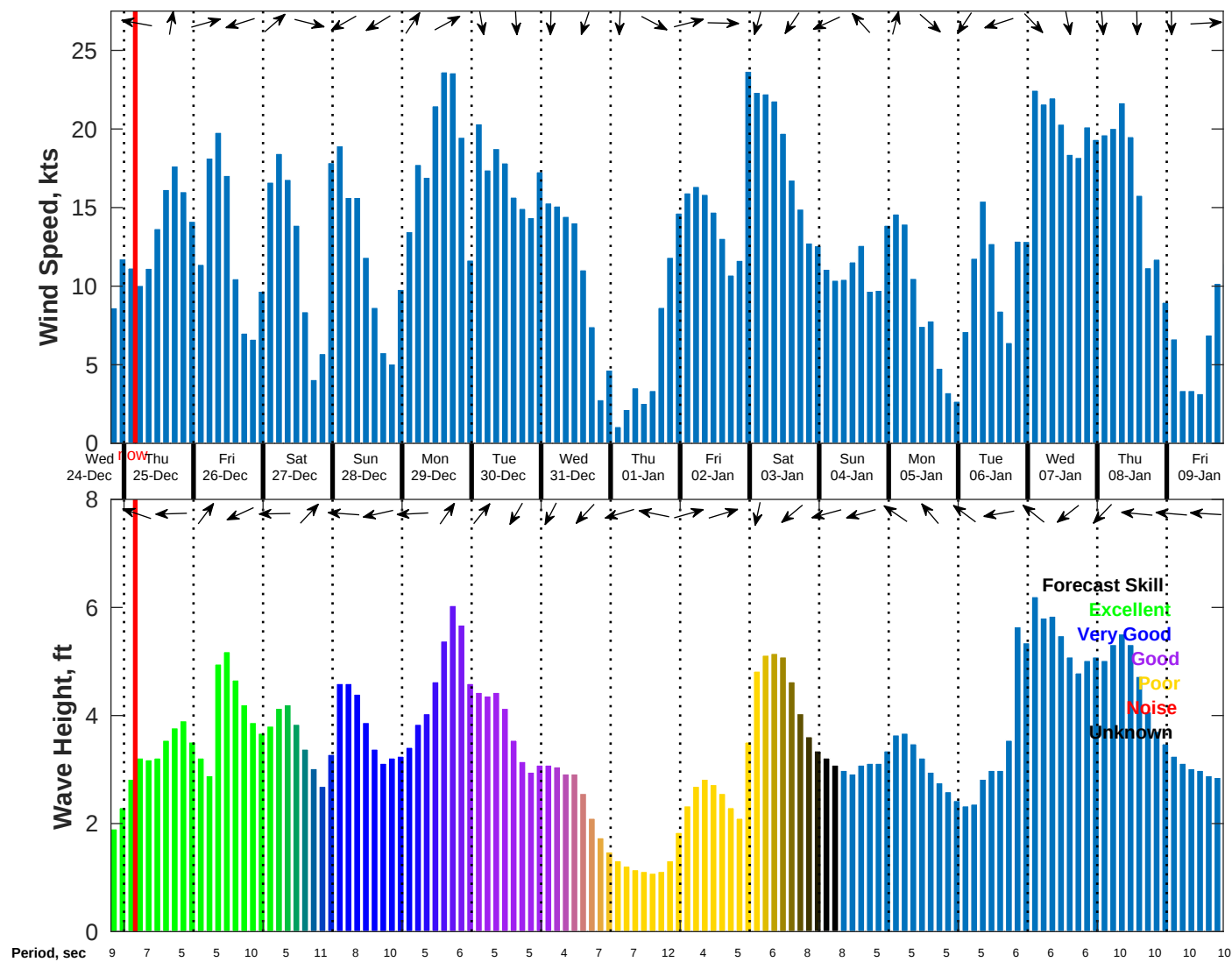
Wind & Wave Forecast for NDBC 41013 from 24-Dec-2025 19:00:00 to 09-Jan-2026 19:00:00
