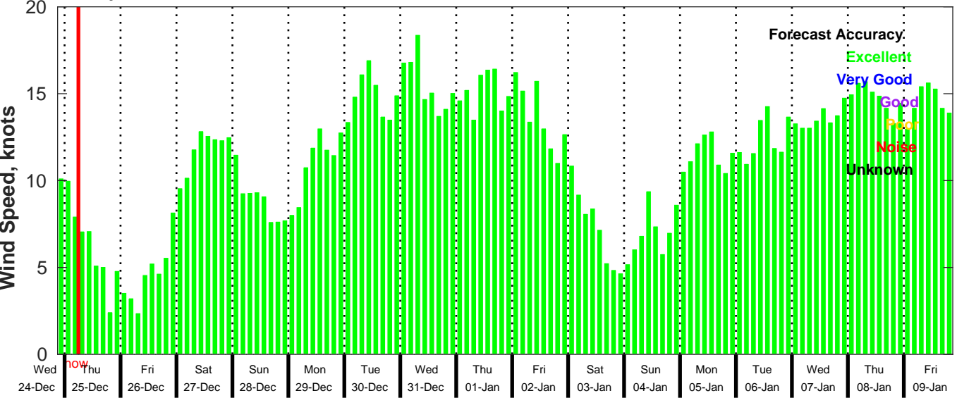
GFS Wind Speed Forecast for NDBC 41040 from 24-Dec-2025 21:00:00 to 09-Jan-2026 21:00:00
