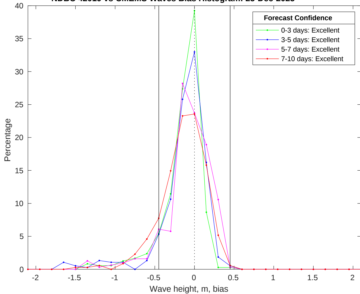
NDBC 42019 vs CMEMS Waves Bias Histogram: 25-Dec-2025
