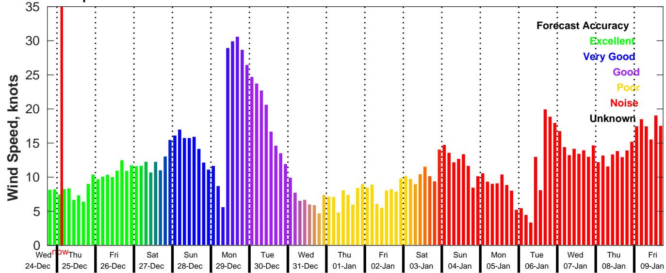
GFS Wind Speed Forecast for NDBC 42019 from 24-Dec-2025 18:00:00 to 09-Jan-2026 18:00:00
