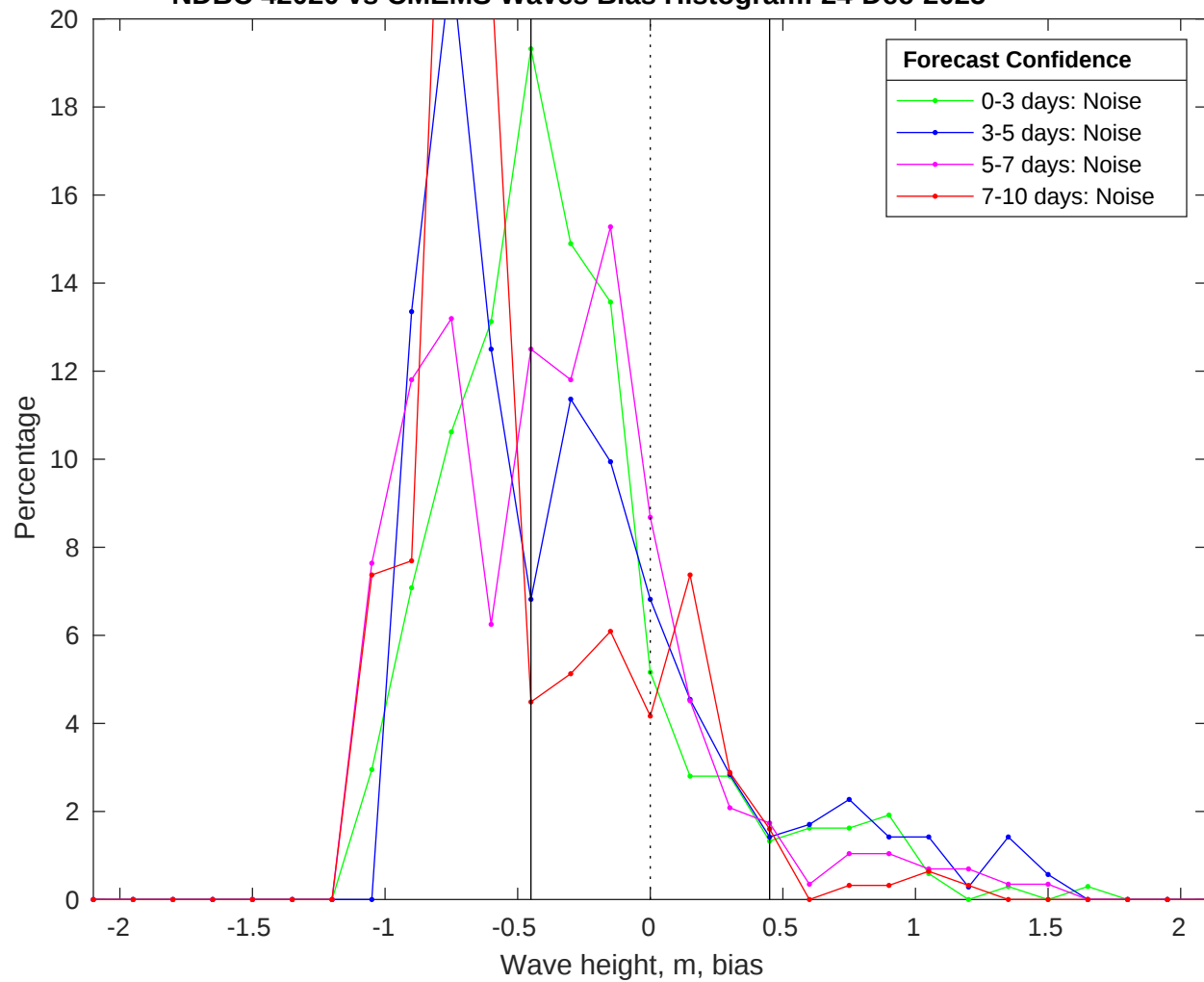
NDBC 42020 vs CMEMS Waves Bias Histogram: 24-Dec-2025
