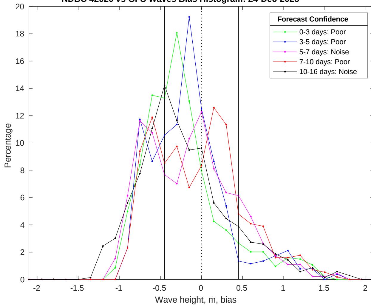
NDBC 42020 vs GFS Waves Bias Histogram: 24-Dec-2025
