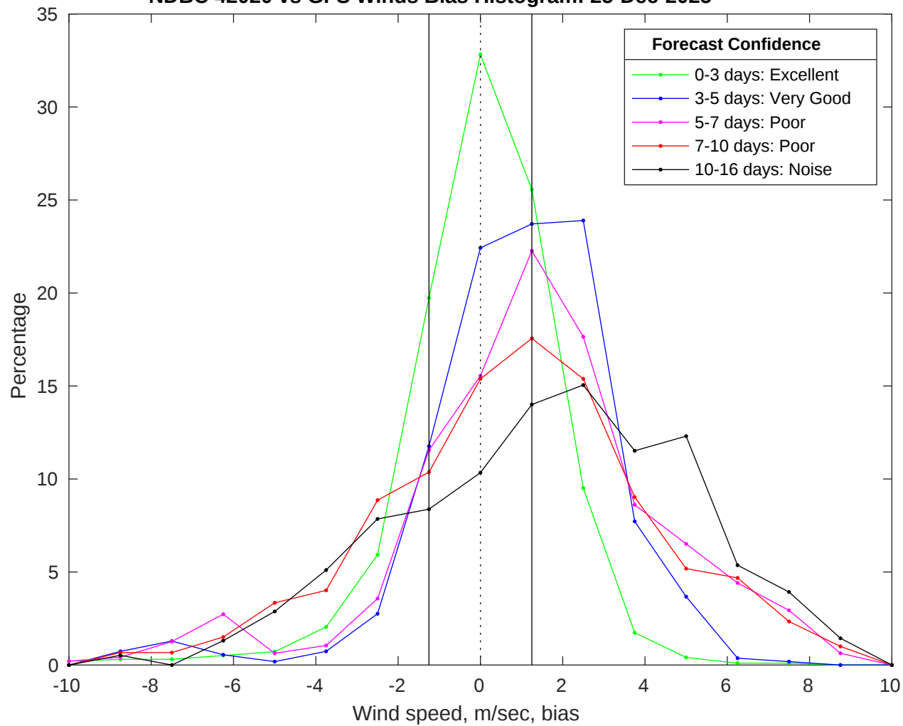
NDBC 42020 vs GFS Winds Bias Histogram: 25-Dec-2025
