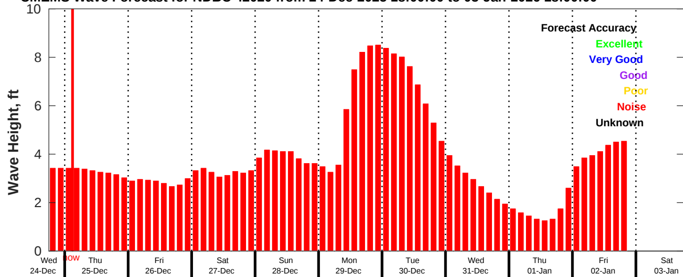
CMEMS Wave Forecast for NDBC 42020 from 24-Dec-2025 18:00:00 to 03-Jan-2026 18:00:00
