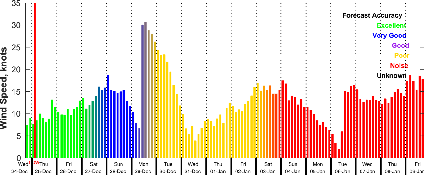
GFS Wind Speed Forecast for NDBC 42020 from 24-Dec-2025 18:00:00 to 09-Jan-2026 18:00:00
