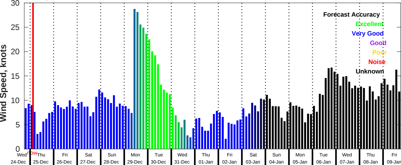
GFS Wind Speed Forecast for NDBC 42035 from 24-Dec-2025 18:00:00 to 09-Jan-2026 18:00:00
