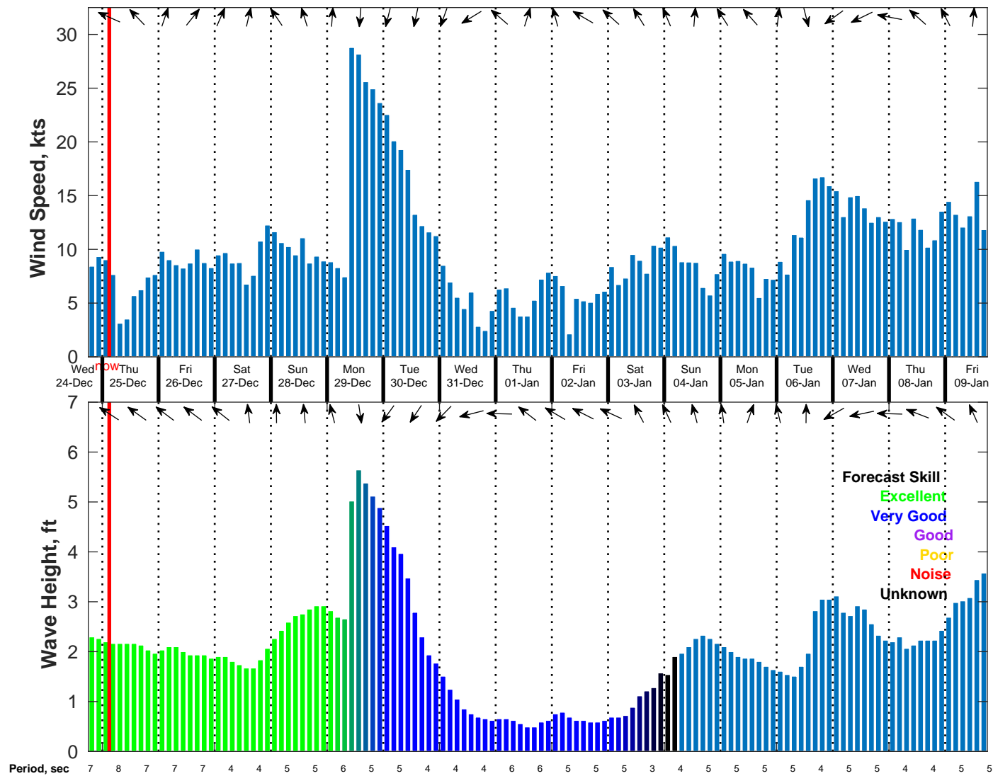
Wind & Wave Forecast for NDBC 42035 from 24-Dec-2025 18:00:00 to 09-Jan-2026 18:00:00
