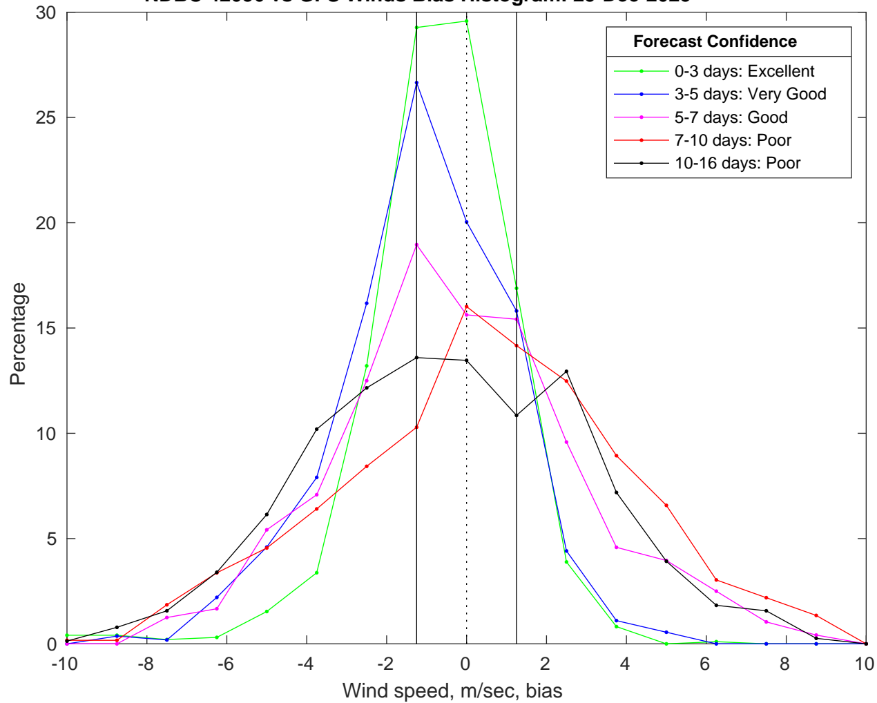
NDBC 42036 vs GFS Winds Bias Histogram: 25-Dec-2025
