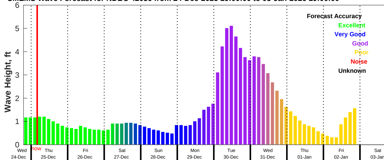
CMEMS Wave Forecast for NDBC 42036 from 24-Dec-2025 19:00:00 to 03-Jan-2026 19:00:00
