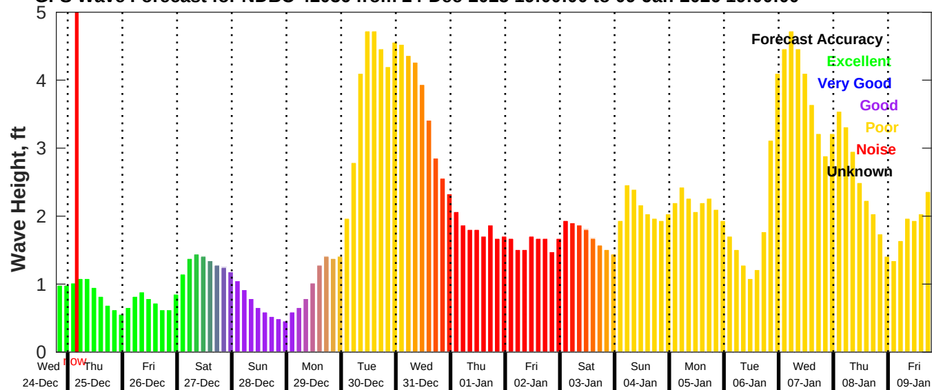
GFS Wave Forecast for NDBC 42036 from 24-Dec-2025 19:00:00 to 09-Jan-2026 19:00:00
