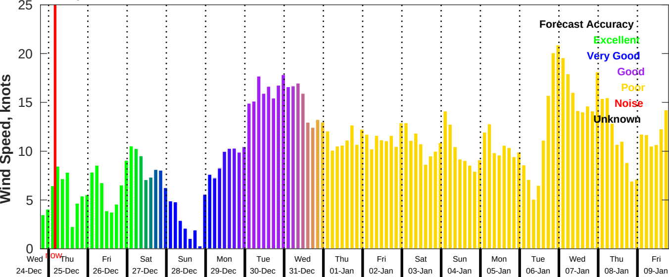
GFS Wind Speed Forecast for NDBC 42036 from 24-Dec-2025 19:00:00 to 09-Jan-2026 19:00:00
