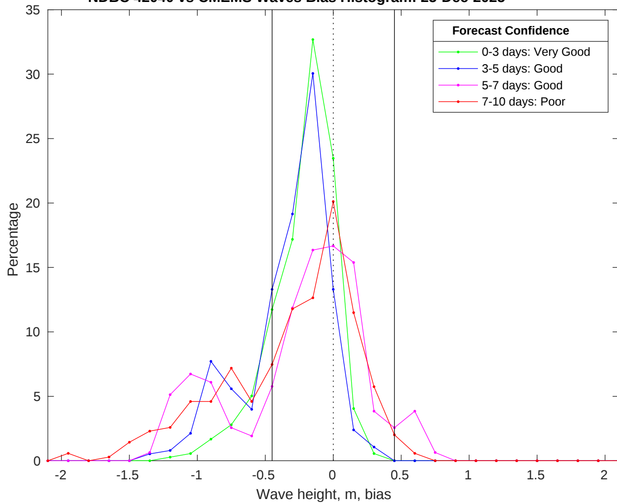
NDBC 42040 vs CMEMS Waves Bias Histogram: 25-Dec-2025
