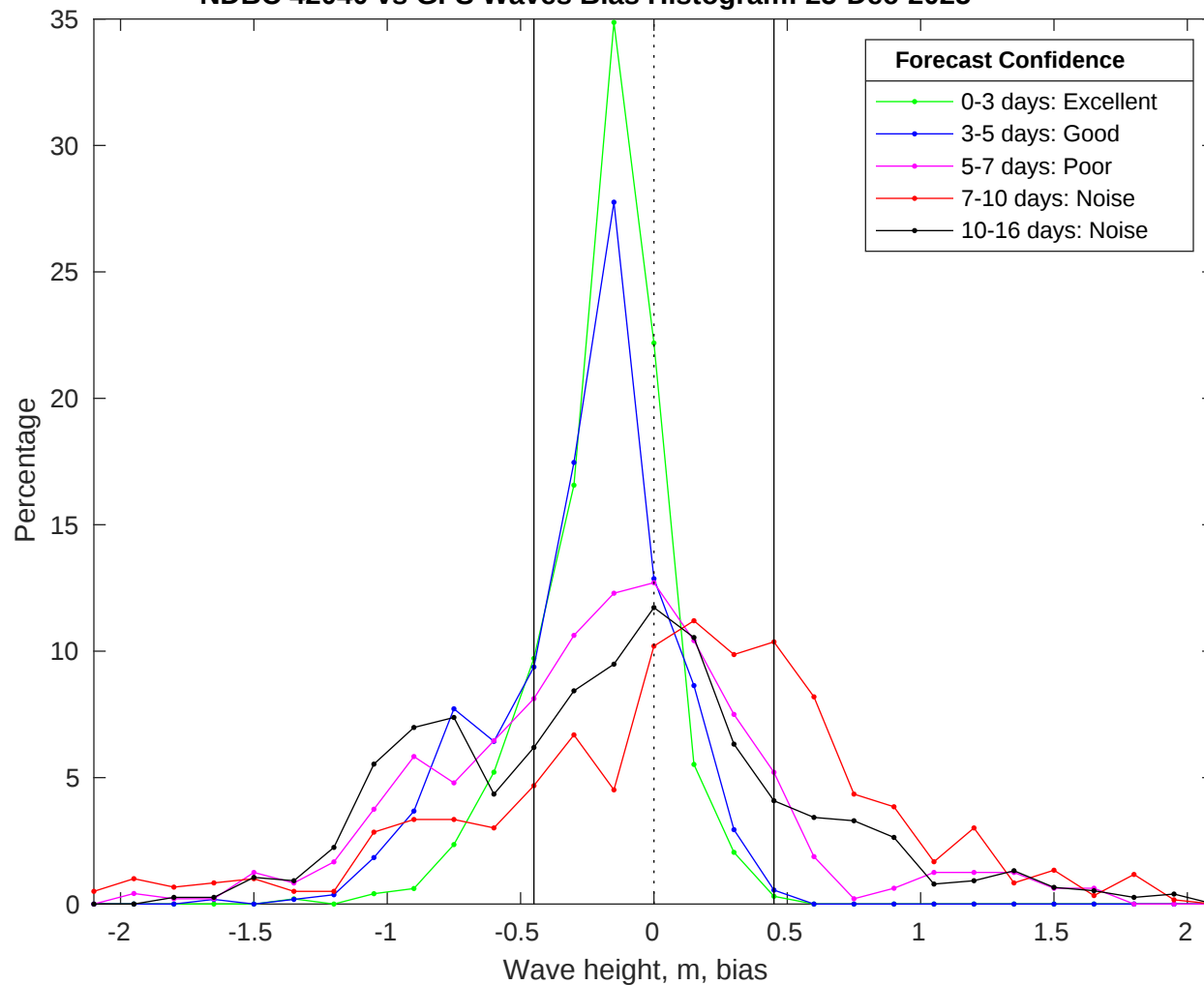
NDBC 42040 vs GFS Waves Bias Histogram: 25-Dec-2025
