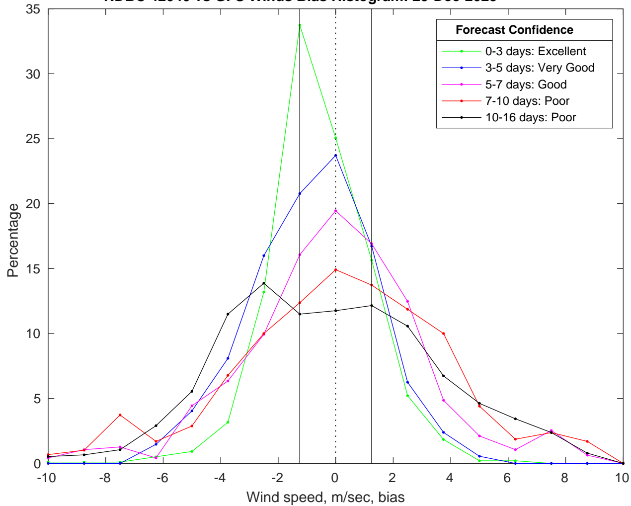
NDBC 42040 vs GFS Winds Bias Histogram: 25-Dec-2025
