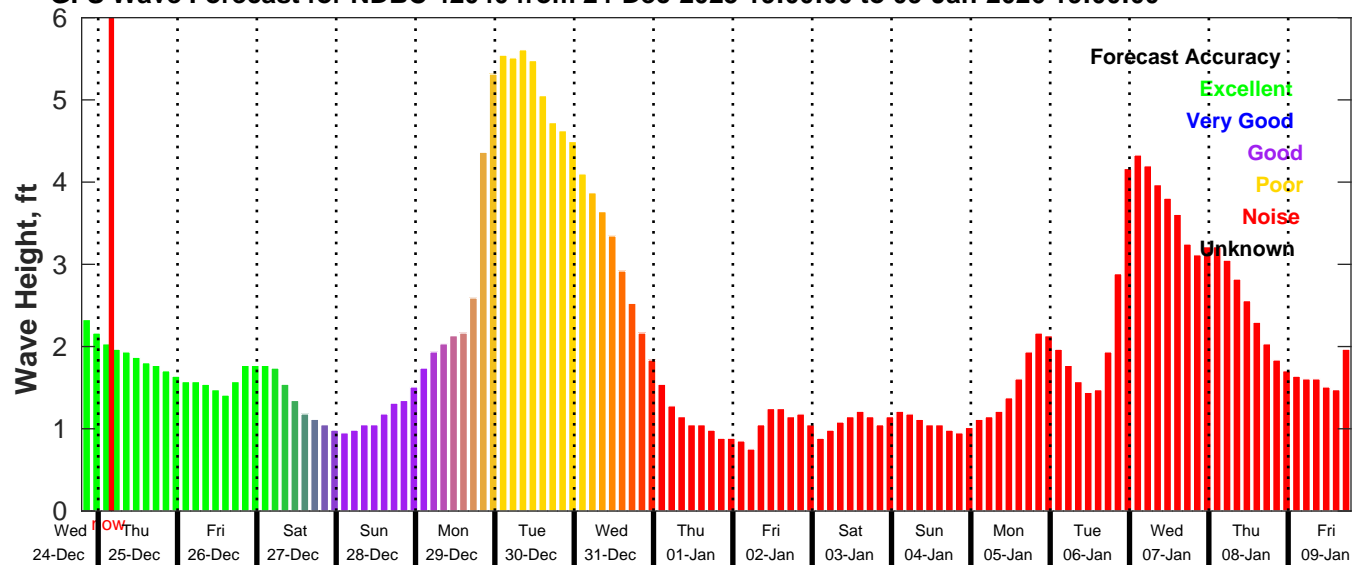
GFS Wave Forecast for NDBC 42040 from 24-Dec-2025 19:00:00 to 09-Jan-2026 19:00:00
