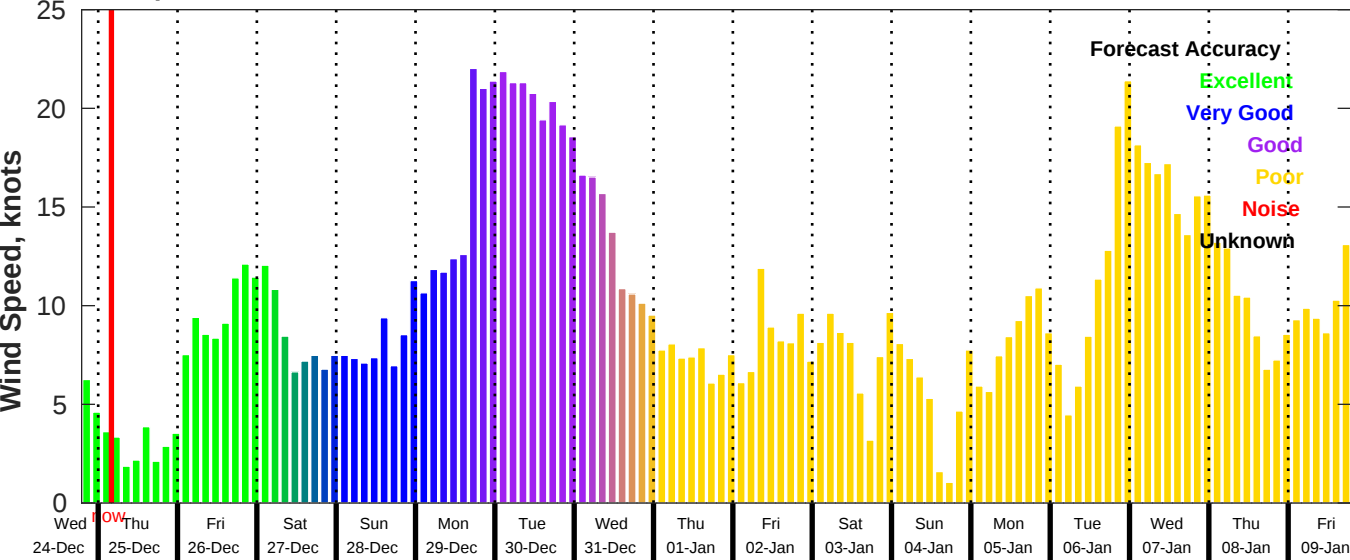
GFS Wind Speed Forecast for NDBC 42040 from 24-Dec-2025 19:00:00 to 09-Jan-2026 19:00:00
