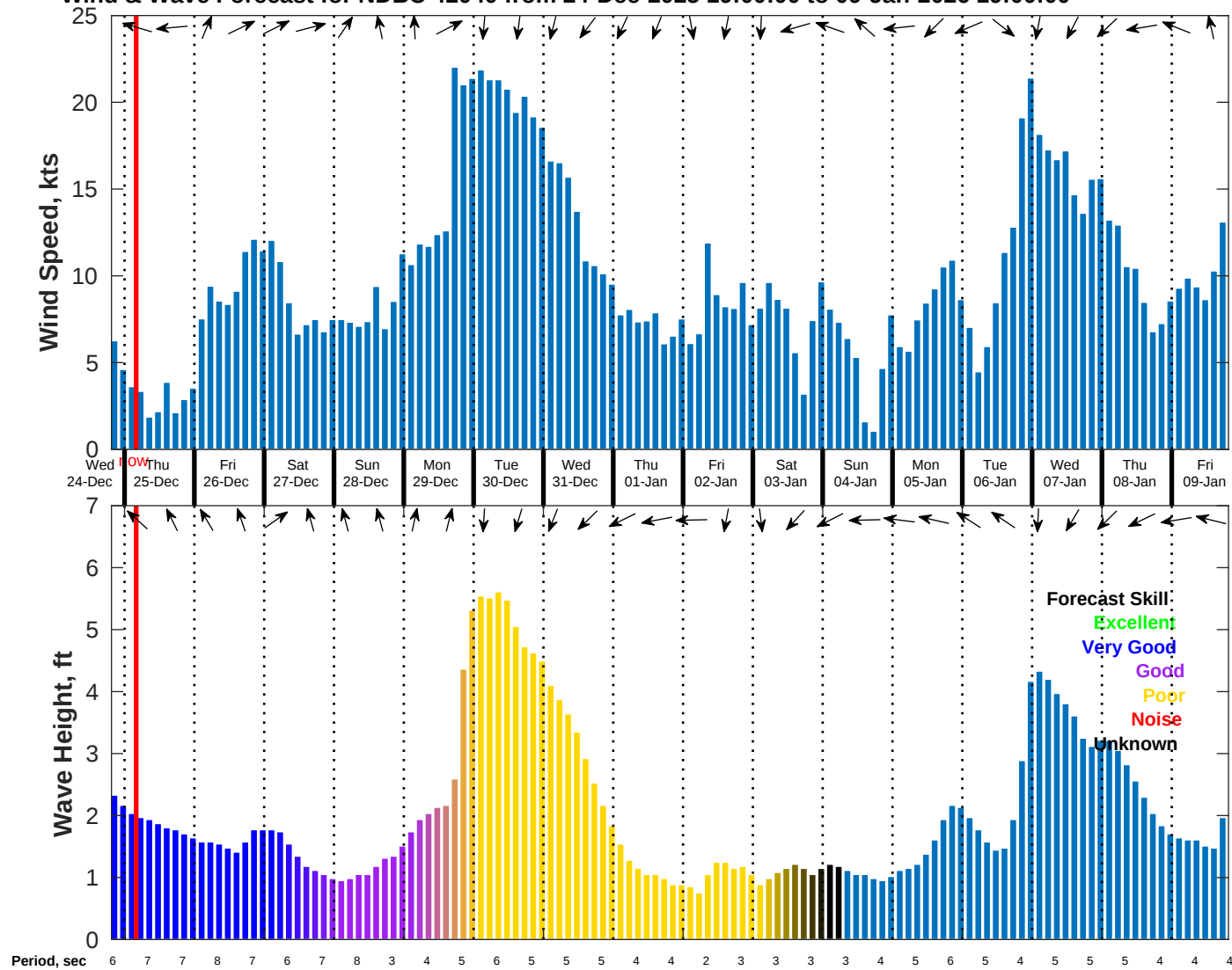
Wind & Wave Forecast for NDBC 42040 from 24-Dec-2025 19:00:00 to 09-Jan-2026 19:00:00
