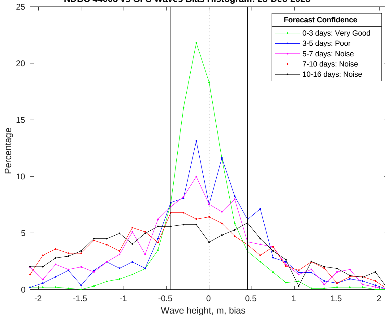
NDBC 44008 vs GFS Waves Bias Histogram: 25-Dec-2025
