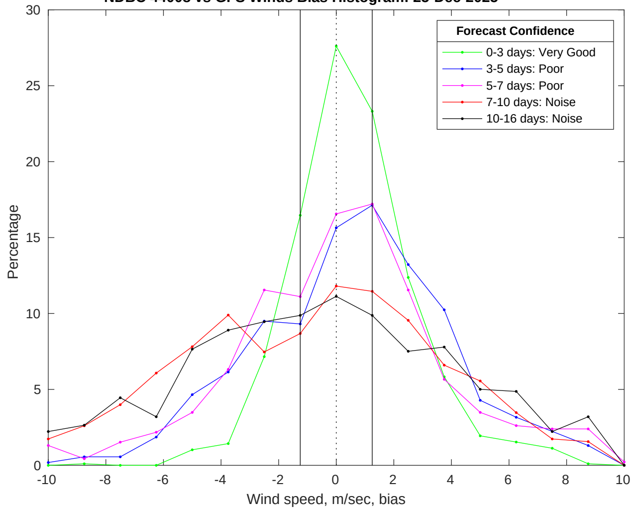
NDBC 44008 vs GFS Winds Bias Histogram: 25-Dec-2025
