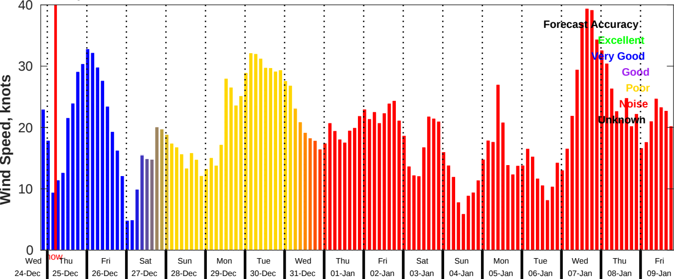
GFS Wind Speed Forecast for NDBC 44008 from 24-Dec-2025 20:00:00 to 09-Jan-2026 20:00:00
