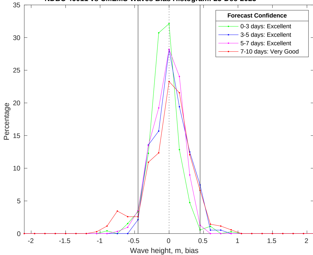
NDBC 46011 vs CMEMS Waves Bias Histogram: 25-Dec-2025
