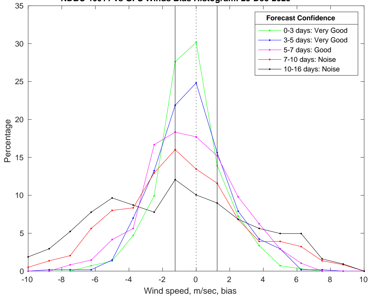
NDBC 46011 vs GFS Winds Bias Histogram: 25-Dec-2025
