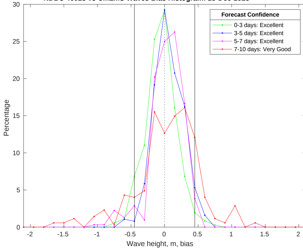
NDBC 46028 vs CMEMS Waves Bias Histogram: 25-Dec-2025
