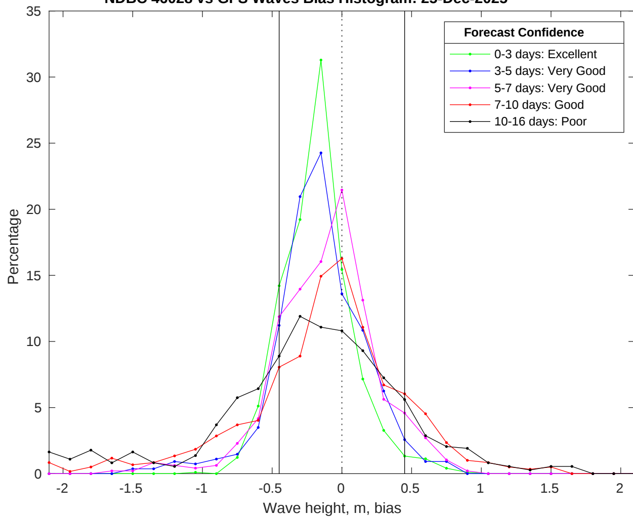
NDBC 46028 vs GFS Waves Bias Histogram: 25-Dec-2025
