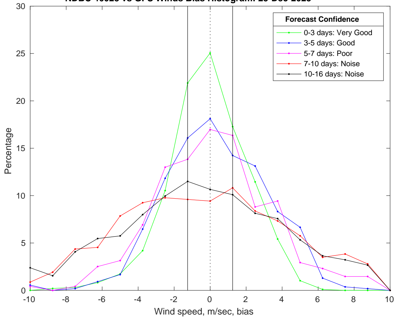
NDBC 46028 vs GFS Winds Bias Histogram: 25-Dec-2025
