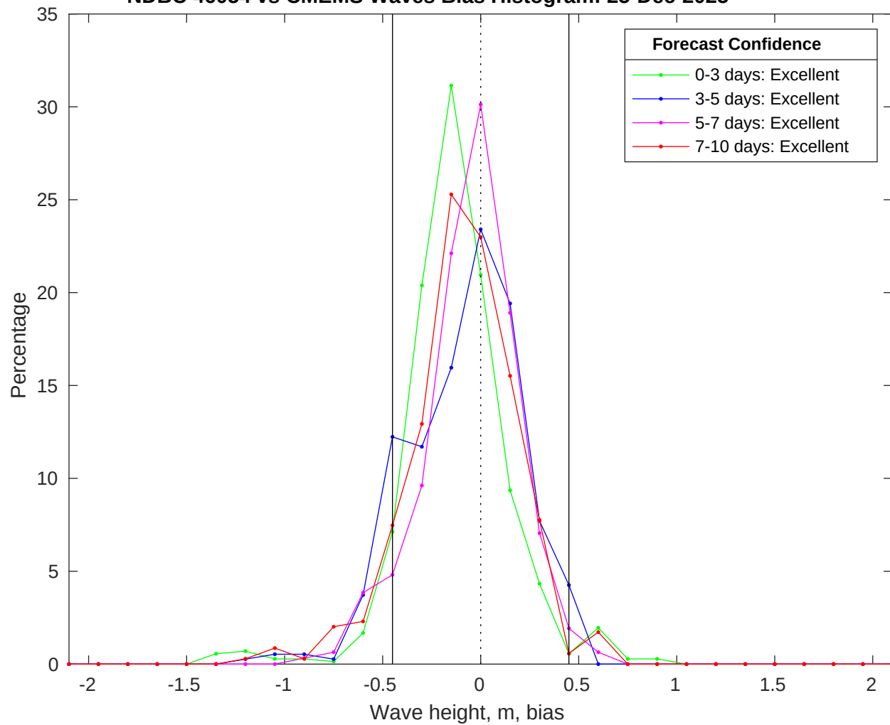
NDBC 46054 vs CMEMS Waves Bias Histogram: 25-Dec-2025
