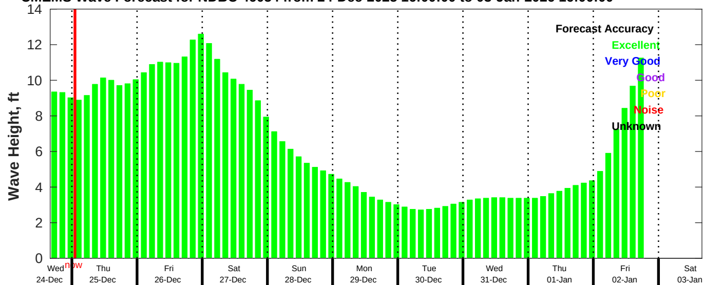
CMEMS Wave Forecast for NDBC 46054 from 24-Dec-2025 16:00:00 to 03-Jan-2026 16:00:00
