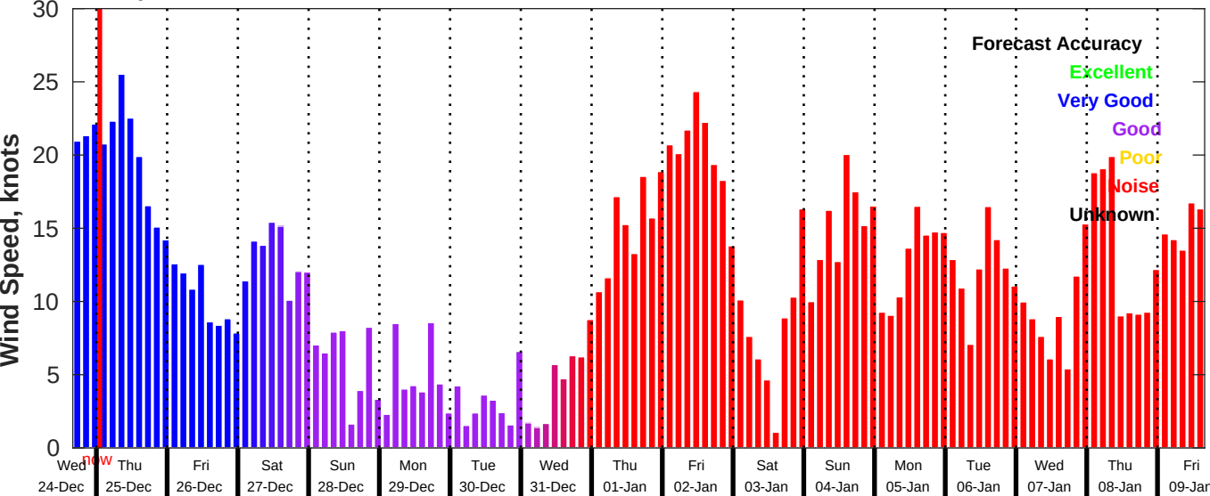
GFS Wind Speed Forecast for NDBC 46054 from 24-Dec-2025 16:00:00 to 09-Jan-2026 16:00:00
